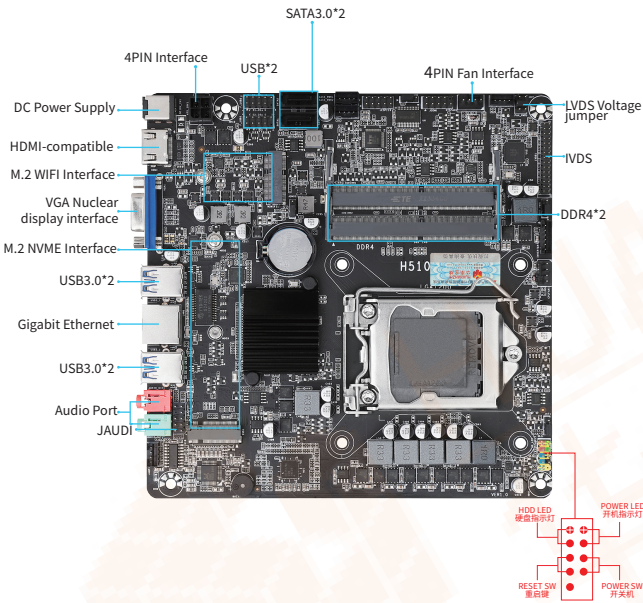
1-1 H510M-I Motherboard Illustration
